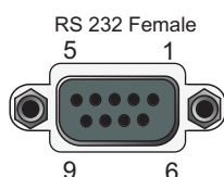
View from solder side
