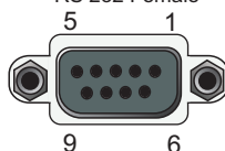
View from solder side
